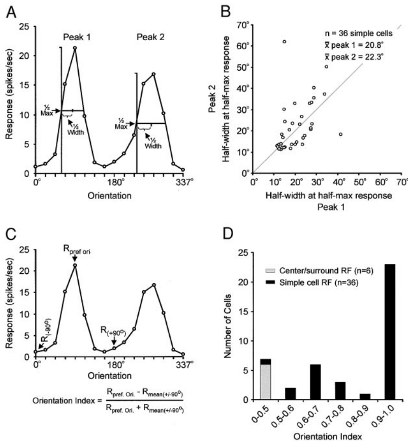
FIG. 4. Simple cells in layer 4 respond selectively to the orientation of a grating stimulus. Orientation-tuning curves were made for individual neurons from responses to gratings presented at 16 different orientations. Orientation-tuning curves were used to assess the tightness of orientation tuning (A), the half width of the peak at half maximum response) and the strength of orientation-selectivity (C, the orientation index). B: mean values for half width at half maximal response were 20.8 \pm 1.2^\circ for primary peaks (peak 1) and 22.3 \pm 2.0^\circ for secondary peaks (peak 2). Peak 2 was defined as the peak response 180 \pm 22^\circ from peak 1. The gray line indicates unit slope. D: orientation index values were typically high among simple cells (mean: 0.86 \pm 0.03 ) and low among neurons with center/surround receptive fields (mean: 0.15 \pm 0.5 ).
