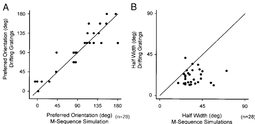
FIG. 7. Comparison of orientation tuning for linear model predictions and neuronal responses to drifting sine wave gratings. A: the optimal orientation (peak in the orientation tuning curve) is shown plotted for the neuronal responses elicited from drifting sine wave gratings vs. model simulations from the best fitting gabor filters to white-noise maps estimated from reverse correlation to m-sequence stimuli. There is a high degree of correlation between the estimates from the neuronal responses and the linear model predictions ( r^2 = 0.85 , P < 0.001 ). B: estimates of orientation tuning bandwidth (half-width at half-height) for the drifting grating responses versus the Gabor filter simulations. On average, the linear model simulation predicts greater orientation tuning bandwidth than those estimated from the drifting gratings responses. The average bandwidth ratio, drifting grating response to simulation, is 1.9 ( P < 0.001 ).
