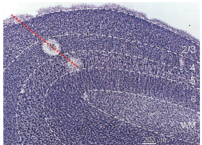
FIG. 1. Photomicrograph of a Nissl-stained section of ferret primary visual cortex. Layer 4 is distinct from layers 2/3 and layer 5 on the basis of cell density and cell size. An electrode track (dashed red line) reconstructed from 2 lesions—1 in layer 4, the other in layer 5—is superimposed on the micrograph.
