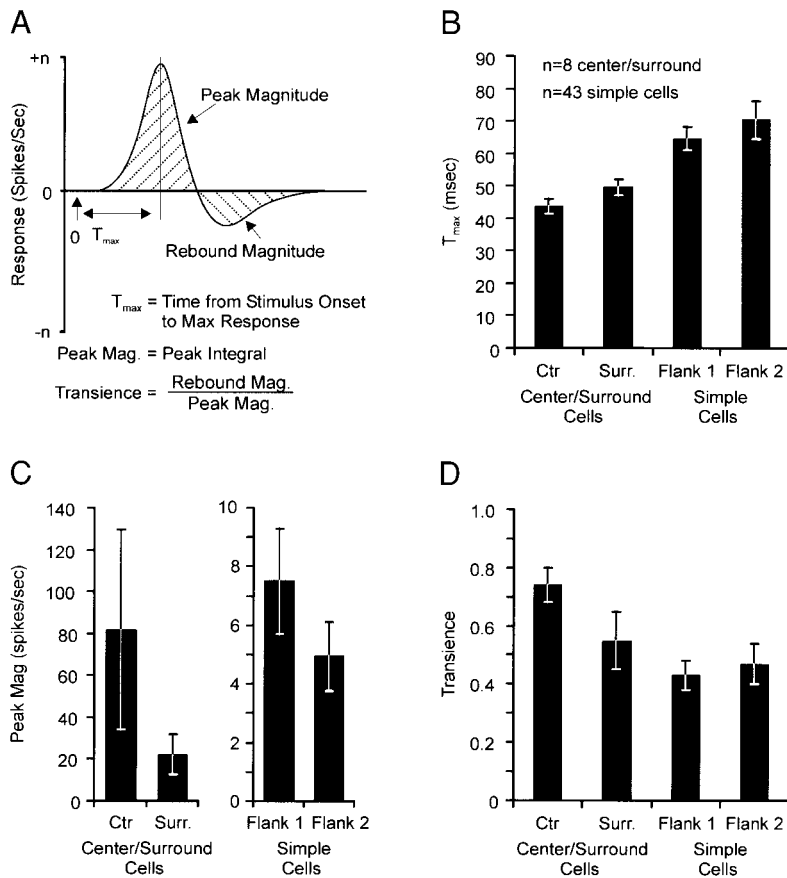
FIG. 3. Comparison of the time course, magnitude, and transience of visual responses of layer 4 neurons. Impulse responses were calculated for each neuron in this study ( n = 51 ). A : diagram illustrating how different features of the impulse response are used to quantify the time course, magnitude, and transience of each neuron's response. B : neurons with center/surround receptive fields typically had shorter latencies between stimulus onset and maximum response ( t_{max} ) than neurons with simple receptive fields. C : peak magnitude was typically greater for neurons with center/surround receptive fields than for neurons with simple receptive fields. D : transience of response was typically greater for neurons with center/surround receptive fields than for neurons with simple receptive fields. Error bars in B-D represent \pm SE.
