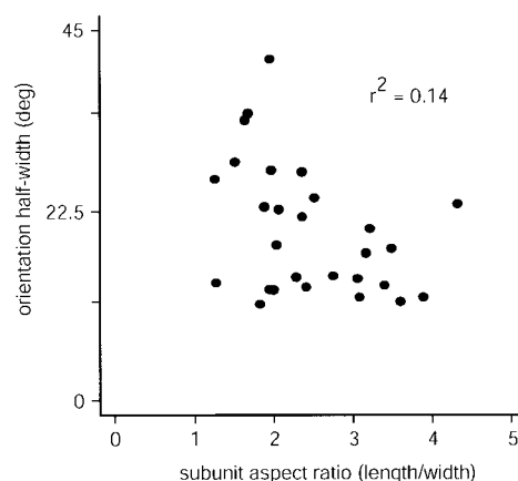
FIG. 9. Orientation tuning half-width vs. receptive-field subunit aspect ratio. Comparison of the orientation tuning curve bandwidth (half-width at half-height) estimated from neuronal spike rates (drifting grating stimulation) with the receptive field subunit aspect ratio (length/width, for the dominant subunit) estimated from the m-sequence reverse correlation 1st-order maps. Although there is no significant correlation between the 2 estimates ( r^2 = 0.14 ), there is a tendency for neurons with higher aspect ratios to have lower peak half widths.
