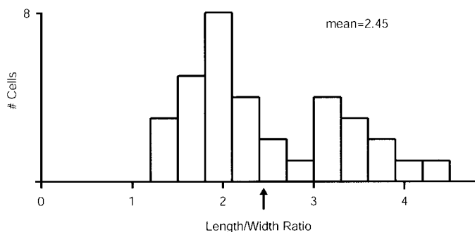
FIG. 8. Length-to-width aspect ratios for simple-cell receptive-field subunits. All estimates are based on m-sequence reverse correlation maps. The raw data were fitted with a Gabor function. The width of the subunits was estimated as the full width at 20% height of the dominant subunit from the fitted Gabors. Lengths were estimated as the full width at 20% height of the Gaussian envelope of the Gabor function. \uparrow , the population mean (2.45).
