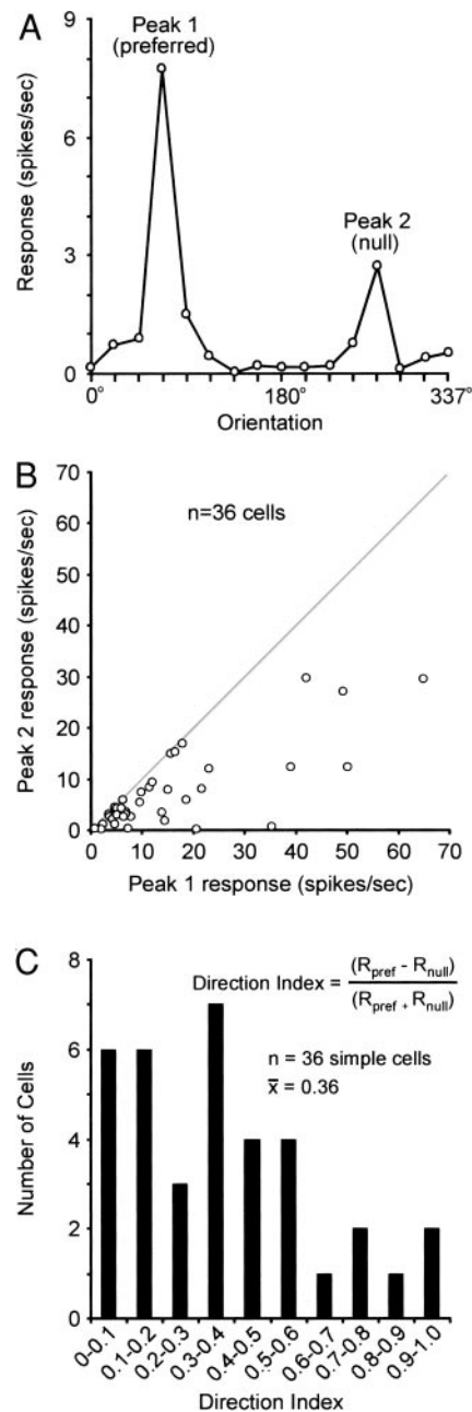
FIG. 5. Direction selectivity of layer 4 neurons. A : peaks in orientation-tuning curves were used to assess the direction selectivity of individual neurons. B : scatter-plot showing the relationship between responses (peak 1, peak 2) to gratings moving in opposite directions. Points falling along the line of unit slope (gray) represent neurons with little or no difference in their response to gratings moving in opposite directions. Neurons below the line of unit slope represent neurons with varying degrees of direction selectivity. C : the direction index was calculated for individual neurons to quantify and compare direction selectivity among simple cells (mean: 0.36 \pm 0.05 ).
