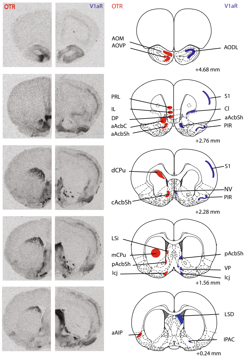
Fig. 1 Representative autoradiograms of OTR and V1aR binding in coronal sections of the brain from the same adult male rat (on the left ) with corresponding rat brain atlas images (Paxinos and Watson 2007; on the right ). Brain regions in which receptor binding was measured are highlighted in red for OTR and are highlighted in blue for V1aR. Distance is measured in millimeters from bregma according to Paxinos and Watson (2007). Note that while many brain regions were analyzed across multiple bregma distances, regions are highlighted in the most representative atlas images only
