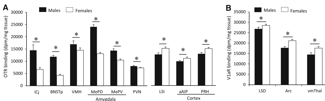
Fig. 6 Brain regions in which OTR a and V1aR b binding densities show sex differences. OTR binding was analyzed on 3-day exposure films for the ICj, BNSTp and VMH and on 9-day exposure films for all other regions. V1aR binding was analyzed on 4-day exposure
